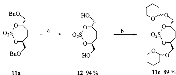
Scheme 3. Reagents and conditions: a: 1 bar H 2 , Pd/C, MeOH, room temp.; b: 3,4-dihydro-2H-pyran, PPTS, CH 2 Cl 2 , room temp., 2 h
