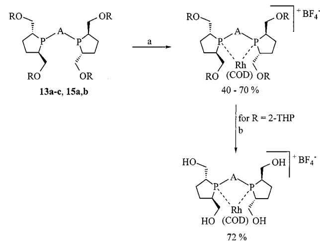
Scheme 5. Reagents and conditions: a: [Rh(COD) 2 ]BF 4 , THF, 0^{\circ}\text{C} to room temp., 1 h; b: aq. HBF 4 , MeOH, room temp., 24 h
