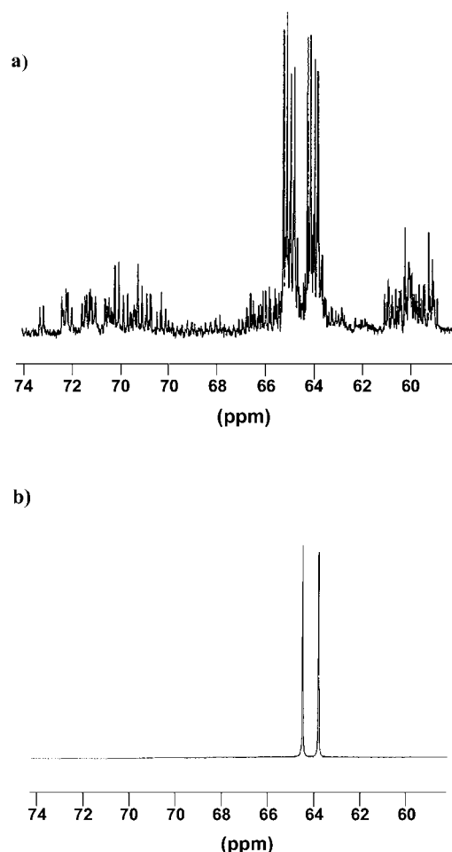
Figure 1. ^{31}\text{P} NMR spectra of [\text{Rh}(\text{COD})(\mathbf{13c})]\text{BF}_4 (a) and [\text{Rh}(\text{COD})(\mathbf{16})]\text{BF}_4 in \text{CDCl}_3 (b)
