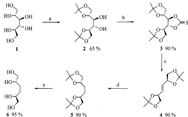
Scheme 1. Reagents and conditions: a: acetone, ZnCl 2 , 25 °C, 2 h; b: S=CCl 2 , DMAP, 0 °C, 1 h; c: P(OEt) 3 , 160 °C, 20 h; d: H 2 , Rh/Al 2 O 3 , THF, room temp. or H 2 , Pt/C, MeOH, room temp.; e: 2 N HCl, 80 °C, 2 h
