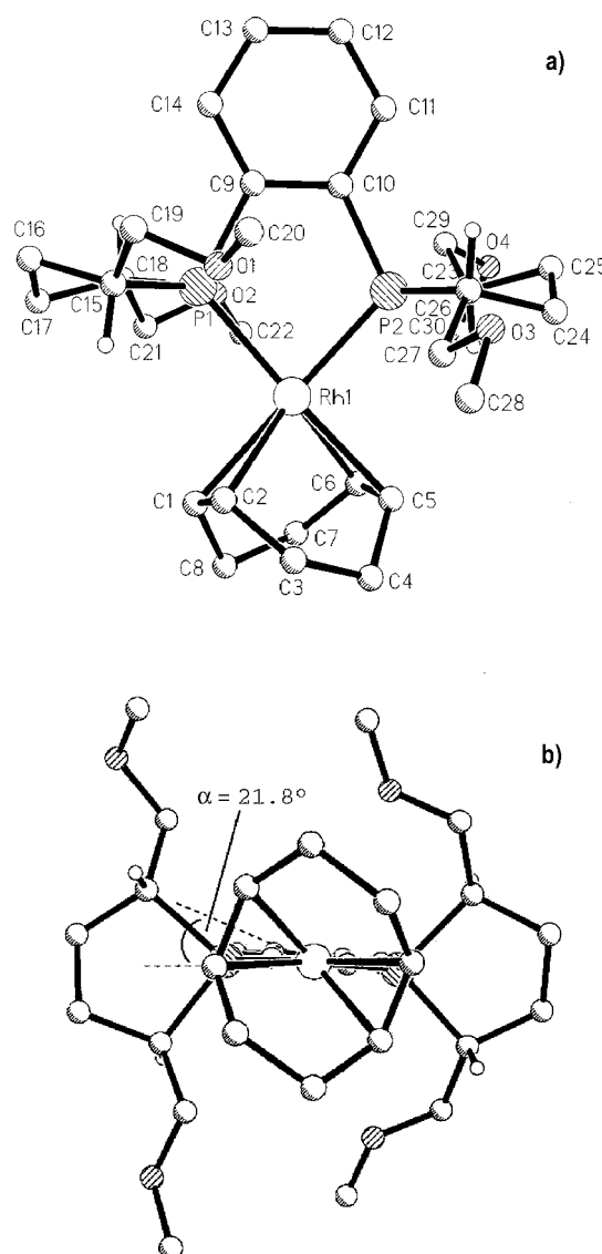
Figure 2. a: top view, showing the 1,2-phenylene unit and the orientation of the methyl oxymethylene group as well as the numbering scheme of [\text{Rh}(\text{COD})(\mathbf{13b})]^+ ; all hydrogen atoms except those that are linked to stereogenic carbon atoms have been omitted for clarity; selected interatomic distances [Å]: Rh1–C1 2.283(4), Rh1–C2 2.207(5), Rh1–C5 2.250(4), Rh1–C6 2.211(4), Rh1–P1 2.285(1), Rh1–P2 2.265(1); selected intramolecular angles ( ^\circ ): P1–Rh1–P2 84.36(4), C1–Rh1–C2 35.5(3), C5–Rh1–C6 35.7(2); b: front view, showing phospholane rings and the dihedral angle between the P–Rh–P plane and the centroid–Rh–centroid plane
