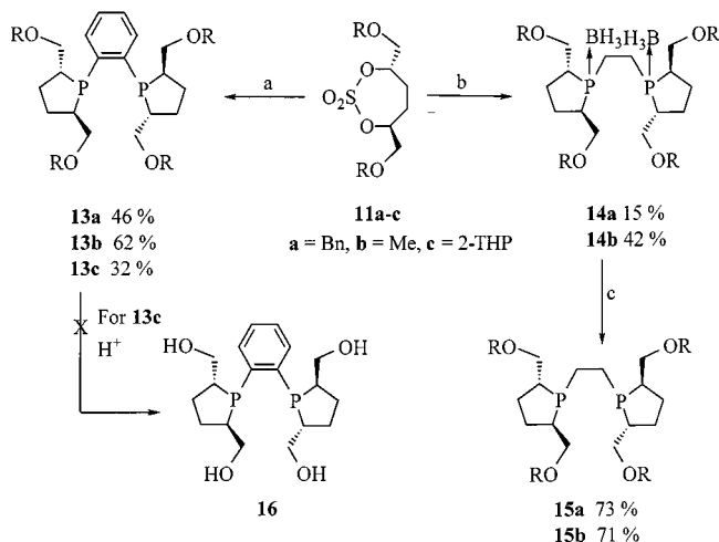
Scheme 4. Reagents and conditions: a: 1. BuLi, THF, -78^{\circ}\text{C} to room temp., 2 h; 2. 1,2-(H 2 P) 2 C 6 H 4 , -78^{\circ}\text{C} to room temp.; 3. BuLi, -78^{\circ}\text{C} to room temp., 12 h; b: 1. BuLi, THF, -78^{\circ}\text{C} to room temp., 2 h; 2. H 3 P-C 2 H 4 -PH 2 , -78^{\circ}\text{C} to room temp.; 3. BuLi, -78^{\circ}\text{C} to room temp., 12 h; 4. BH 3 -THF, -10^{\circ}\text{C} to room temp., 2 h; c: DABCO, toluene, 40^{\circ}\text{C}
