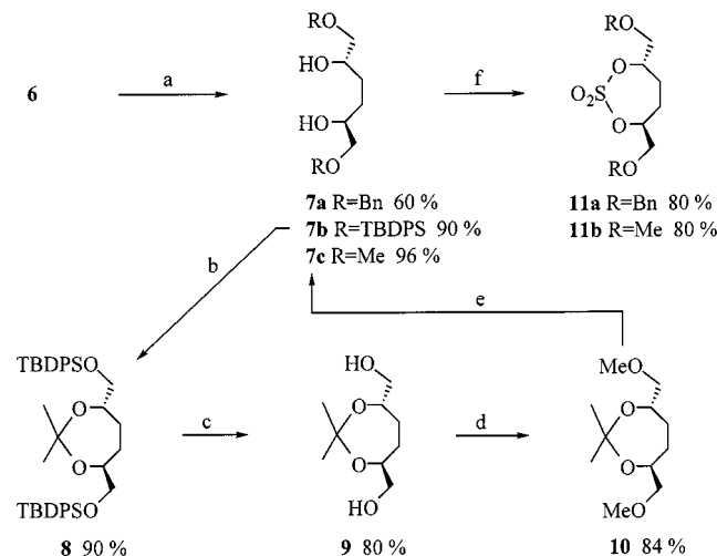
Scheme 2. Reagents and conditions: a: for 7a : 1. Bu 2 Sn=O, toluene, reflux, 4 h; 2. Bu 4 NBr, BnBr, toluene, reflux, 16 h; for 7b : TBDPS-Cl, imidazole, DMF, 0 °C to room temp., 24 h; b: 2-methoxypropene, TsOH, 0 °C, 1 h; c: TBAF, THF, room temp., 2 h; d: NaH, MeI, THF, room temp., 16 h; e: 1 N HCl, THF, room temp., 1 h; f: SOCl 2 , CCl 4 , reflux, 1.5 h; 2. RuCl 3 , NaIO 4 , CCl 4 , CH 3 CN, H 2 O, 0 °C to room temp., 1 h
